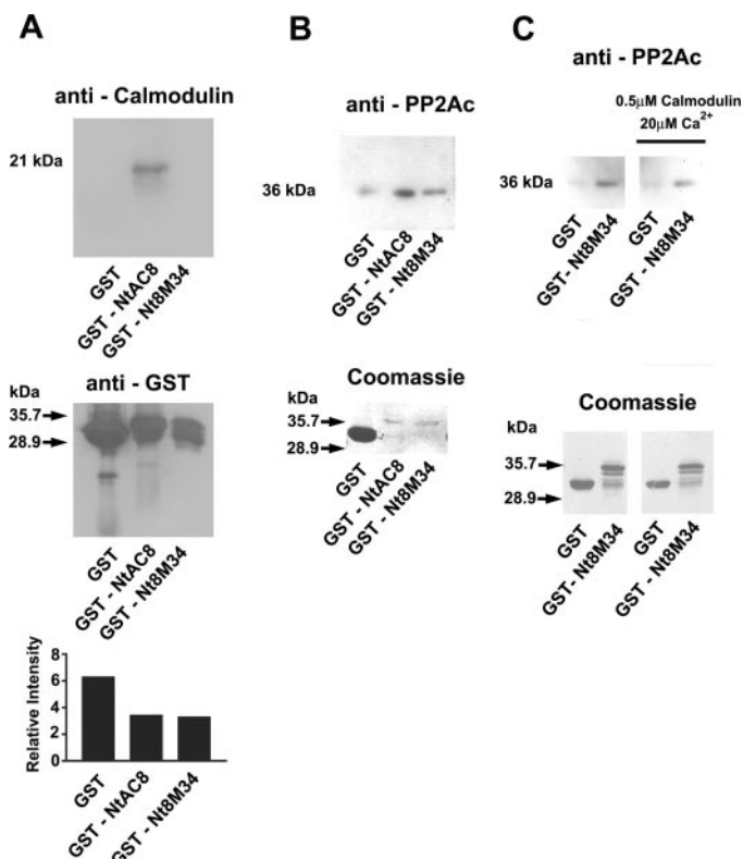
Fig. 5. Amino acids critical for \text{Ca}^{2+} /calmodulin association are not essential for binding \text{PP2A}_C . A , GST, a GST fusion protein containing the full-length N terminus of AC8, or a GST fusion protein containing the full-length N terminus of AC8 with point mutations in the calmodulin binding region (8M34) that were immobilized on glutathione-Sepharose beads were incubated in the presence or absence of 20 \mu\text{M} \text{Ca}^{2+} and 0.5 \mu\text{M} calmodulin. After washing with 1% Triton X-100, the pull-downs were resolved by SDS-PAGE and immunoblotted with an antibody raised against calmodulin (anti-calmodulin). The same blot stripped and reprobed with an antibody raised against GST (anti-GST) is shown at the bottom. The relative amount of the three fusion proteins was quantified by densitometric analysis of the GST immunoblot. B , GST fusion proteins containing the full-length N terminus of AC8 or the full-length N terminus of AC8 with point mutations in the calmodulin binding region (8M34) immobilized on glutathione-Sepharose beads were incubated with equivalent volumes of GST precleared brain membranes. The affinity precipitates were resolved by SDS-PAGE and immunoblotted with an antibody raised against the catalytic subunit of protein phosphatase 2A (anti- \text{PP2A}_C ). The Coomassie-stained membrane is shown at the bottom. C , a GST fusion protein containing the full-length N terminus of AC8 with point mutations in the calmodulin binding region (8M34) immobilized on glutathione-Sepharose beads was incubated with GST precleared brain membranes containing either 1 mM EDTA/EGTA or 20 \mu\text{M} \text{Ca}^{2+} and 0.5 \mu\text{M} calmodulin. The affinity precipitates were resolved by SDS-PAGE and were immunoblotted with an antibody raised against the catalytic subunit of protein phosphatase 2A (anti- \text{PP2A}_C ). The Coomassie-stained membrane is shown at the bottom.
