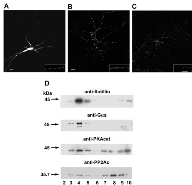
Fig. 7. AC8 and \text{PP2A}_C are present in lipid rafts. Hippocampal neurons at 10 DIV 48 h after transfection with GFP ( A ) or GFP-AC8 ( B ). C , hippocampal neurons at 10 DIV 48 h after transfection with GFP-AC8 were extracted with 0.5% Triton X-100 at 4^\circ\text{C} . The scale bar in all images represents 10 \mu\text{M} . D , crude mouse forebrain membranes were incubated in cold Triton X-100 at a 10:1 detergent-to-protein ratio and prepared for sucrose equilibrium density gradient centrifugation as described under Materials and Methods . Fractions (3–10) were resolved by SDS-PAGE and immunoblotted with antibodies raised against flotillin (anti-flotillin), PKA catalytic subunit (anti-PKA), \text{G}\alpha_{\text{s}} -olf (anti- \text{G}\alpha_{\text{s}} ), or the catalytic subunit of protein phosphatase 2A (anti- \text{PP2A}_C ).
