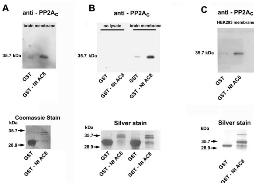
Fig. 1. The N terminus of AC8 interacts with the catalytic subunit of protein phosphatase 2A. Mouse cortical membranes were solubilized by either 1% NP40 (A) or 2% SDS (B), precleared with an excess of GST, and incubated with a GST fusion protein containing the full-length N terminus of AC8 immobilized on glutathione-Sepharose beads. The affinity precipitates were resolved by SDS-PAGE and were immunoblotted with an antibody raised against the catalytic subunit of protein phosphatase 2A (anti-PP2A C ). Aliquots from the same experiments were examined for protein loading by Coomassie staining of membranes or parallel in-gel silver nitrate staining. C, HEK293 membranes were solubilized by 2% SDS, precleared with an excess of GST, and incubated with a GST fusion protein containing the full-length N terminus of AC8 immobilized on glutathione-Sepharose beads. The affinity precipitates were resolved by SDS-PAGE and were immunoblotted with an antibody raised against the catalytic subunit of protein phosphatase 2A (anti-PP2A C ). Aliquots from the same experiments were examined for protein loading by parallel in-gel silver nitrate staining.
