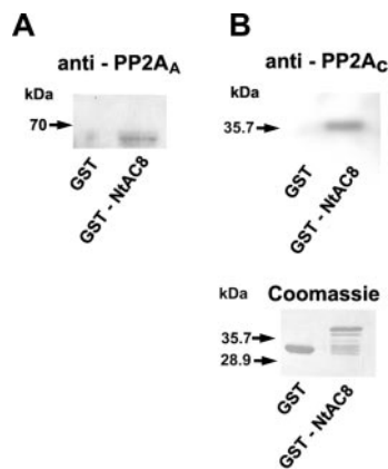
Fig. 2. The N terminus of AC8 interact with the PP2A core enzyme. A GST fusion protein containing the full-length N terminus of AC8 immobilized on glutathione-Sepharose beads was incubated with GST pre-cleared brain membranes. The affinity precipitates were resolved by SDS-PAGE and immunoblotted with an antibody raised against the scaffolding subunit of protein phosphatase 2A (anti-PP2A A ) (A) or an antibody raised against the catalytic subunit of protein phosphatase 2A (anti-PP2A C ) (B). The Coomassie-stained membrane is shown at the bottom.
