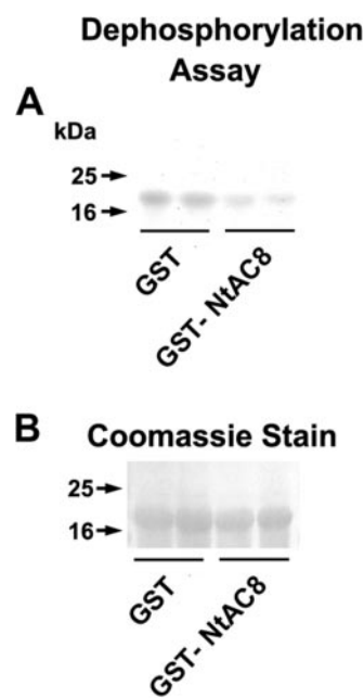
Fig. 3. The N terminus of AC8 interacts with catalytically active PP2A C . GST or a GST fusion protein containing the full-length N terminus of AC8 immobilized on glutathione-Sepharose beads was incubated with Triton X-100-solubilized HEK293 cell lysates. The resulting washed affinity precipitates were incubated with myelin basic protein that had been previously phosphorylated with the catalytic subunit of PKA in buffer containing [ \gamma - 32 P]ATP. A, proteins were resolved by SDS-PAGE and the level of myelin basic protein dephosphorylation determined by autoradiography. B, the Coomassie-stained membrane is shown at the bottom.
