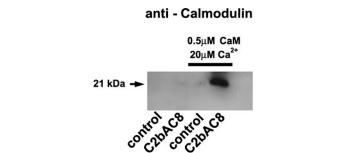
Fig. 6. The calmodulin binding domains of AC8 are not regulated by phosphorylation. Cobalt affinity gel (control) or a histone-fusion protein containing the C terminus of AC8 immobilized on cobalt affinity gel (C2bAC8) was incubated in the presence or absence of 20 \mu\text{M} \text{Ca}^{2+} and 0.5 \mu\text{M} calmodulin. The affinity precipitates were resolved by SDS-PAGE and immunoblotted with an antibody raised against calmodulin (anti-calmodulin). The Coomassie-stained membrane is shown at the bottom.
