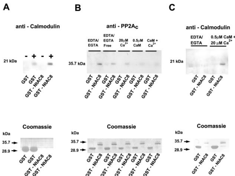
Fig. 4. A competitive interaction between Ca 2+ /calmodulin and PP2A C for association with the N terminus of AC8. A, GST or GST fusion proteins containing the full-length N terminus of AC8 immobilized on glutathione-Sepharose were incubated in the absence (–) or presence (+) of 0.5 \mu M calmodulin and 20 \mu M Ca 2+ . The pull-downs were resolved by SDS-PAGE and immunoblotted with an antibody raised against calmodulin (anti-calmodulin). The Coomassie-stained membrane is shown at the bottom. B, a GST fusion protein containing the full-length N terminus of AC8 immobilized on glutathione-Sepharose beads was incubated with GST-purified brain membranes containing either 1 mM EDTA/EGTA, no exogenous additions, 20 \mu M Ca 2+ , 0.5 \mu M calmodulin, or 20 \mu M Ca 2+ and 0.5 \mu M calmodulin. The affinity precipitates were resolved by SDS-PAGE and immunoblotted with an antibody raised against the catalytic subunit of protein phosphatase 2A (anti-PP2A C ). The Coomassie-stained membrane is shown at the bottom. C, a GST fusion protein containing the full-length N terminus of AC8 immobilized on glutathione-Sepharose beads was incubated with GST-purified brain membranes containing either 1 mM EDTA/EGTA or 20 \mu M Ca 2+ and 0.5 \mu M calmodulin. The affinity precipitates were resolved by SDS-PAGE and immunoblotted with an antibody raised against calmodulin (anti-calmodulin). The Coomassie-stained membrane is shown at the bottom.
